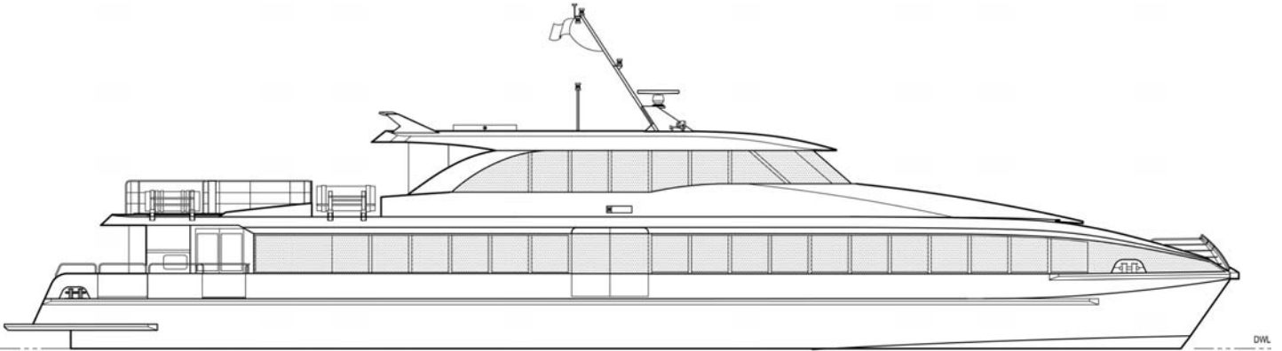
OUTBOARD PROFILE
