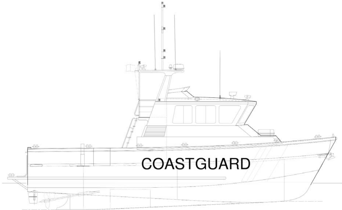
OUTBOARD PROFILE
