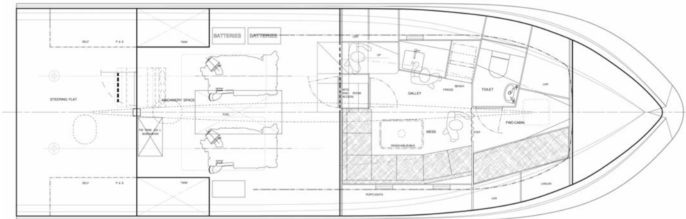
MAIN DECK
