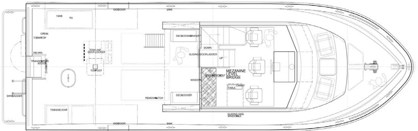
UPPER DECK
